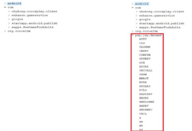
Original code of the APK on the left, versus injected APK on the right
